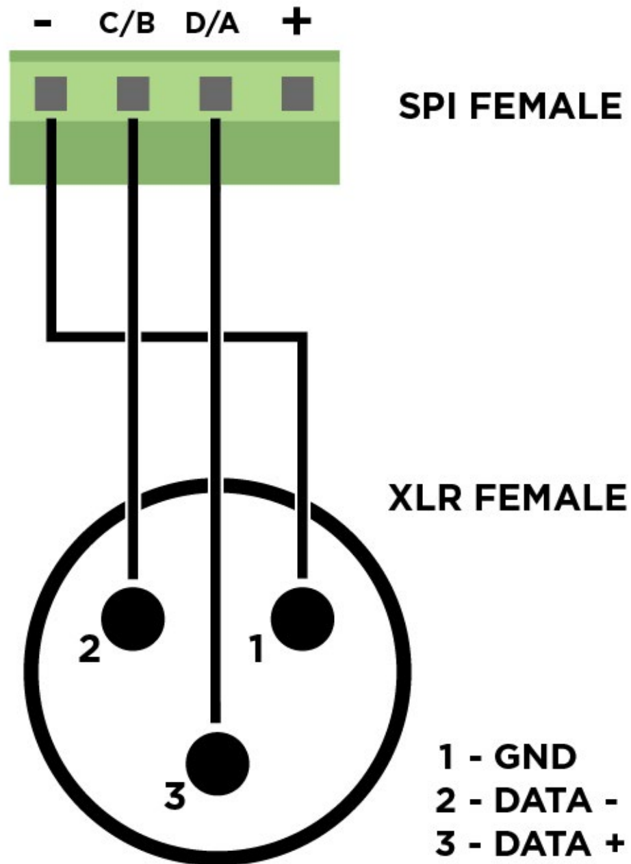
SPI to DMX XLR, Female to female, Adapter Cable schematic diagram
